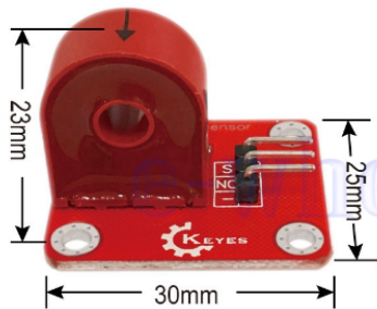
Gambar 2. Sensor Arus TA12-200
