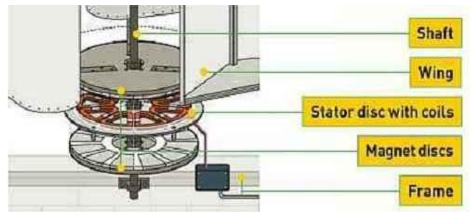
Gambar 5. Skema turbin angin (vertical axis wind turbine)
