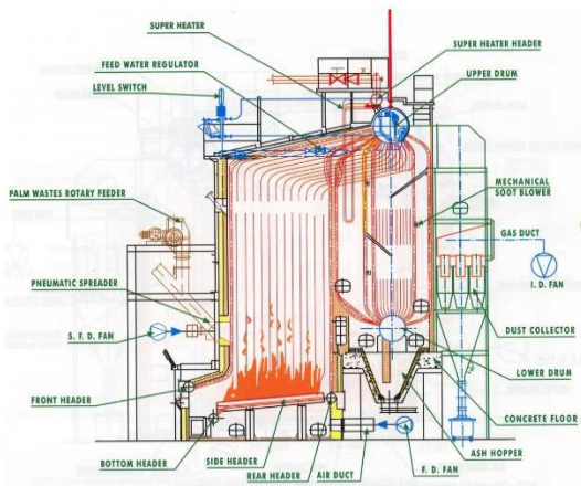
Gambar 2.1. Water Tube boiler
