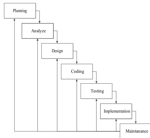
Gambar 1. Model Waterfall
